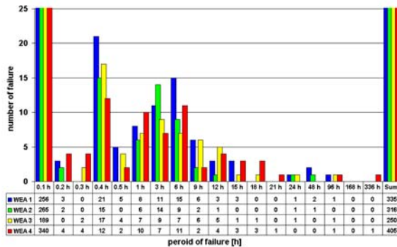
Fig. 8: The Analysis of the duration of downtimes shows how long the turbine, the technical wind farm operator and the service team of the manufacturer need to eliminate the errors.
