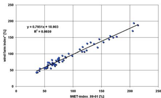
Fig. 10: Correlation analysis between the monthly energy production of a wind farm and the IWET-production index.
