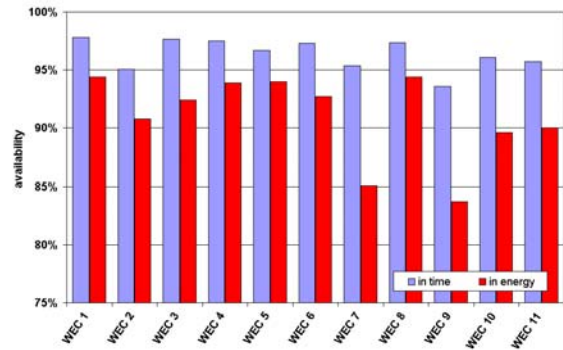
Fig. 9: Presentation of availability regarding time and energy yield
