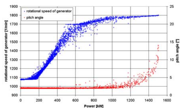
Fig. 1: Raw data of generator speed and pitch angle as function of active power (for noise optimised operation).
