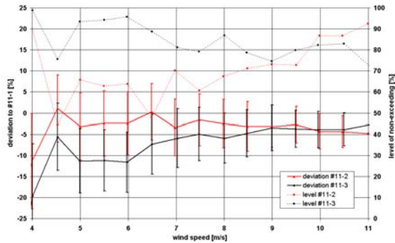
Fig. 6: Relative comparison between power curves of the same turbine for three different control settings.
