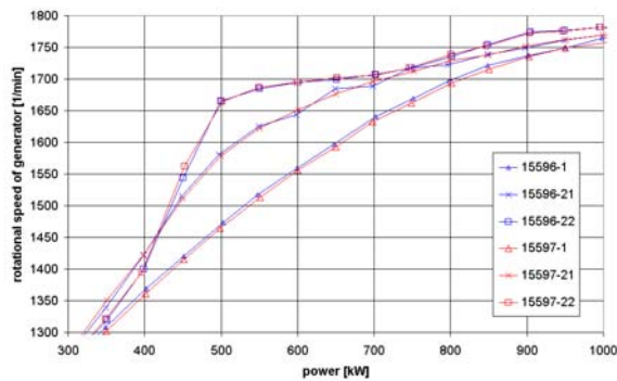
Fig. 2: Bin analysed rotor speed control. In this example three different states of the turbines were identified.
