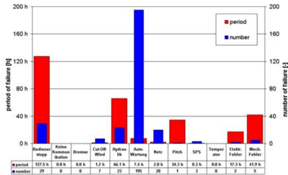
Fig. 7: Analysis of occurrence of error causes.
