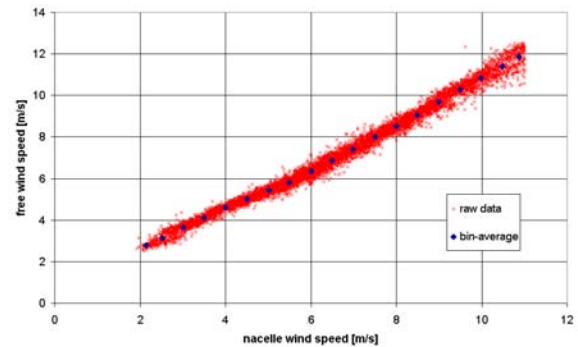
Fig. 3: Correction of wind speed measured at the nacelle to the free wind speed, evaluation from SCADA-data by assuming the guaranteed power curve to be valid.
